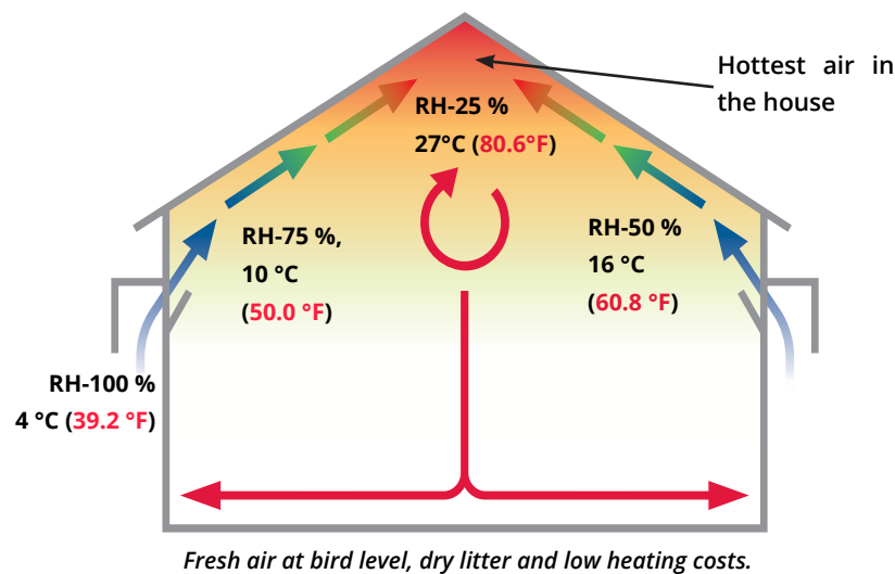
Ideal air flow and air mixing
