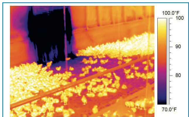
Fans or windows don't have the same insulation capacity as the walls. They can create uncomfortable areas for the birds.
