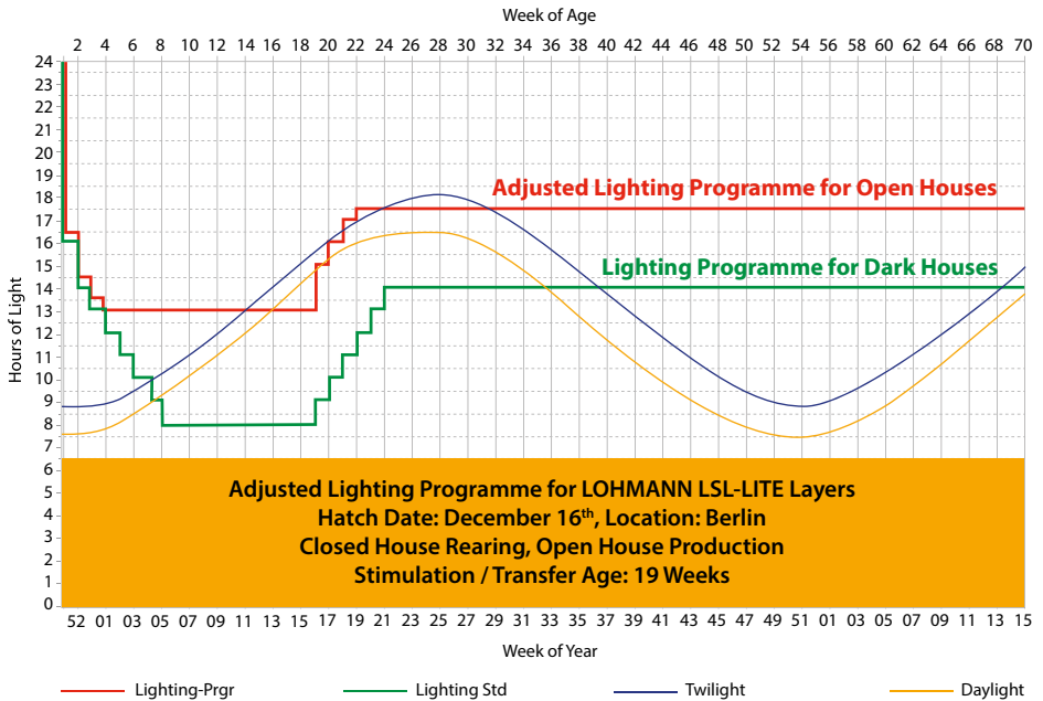
An example of a lighting programme for LOHMANN LSL-LITE Layers adjusted to location, condition and requirements by LOHMANN lighting programme tool
