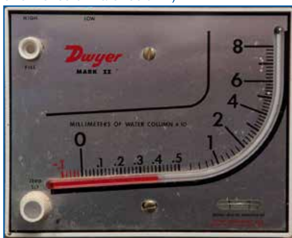
Figure 103: A manometer used to monitor air pressure within the house (the reading given is equivalent to 0.15 inches of water column).
