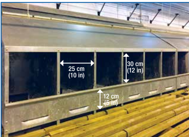
Figure 52: Nest box entrance dimensions.
