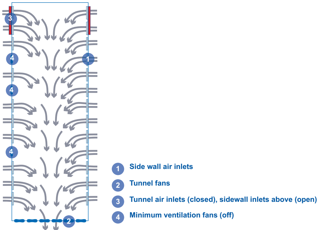
Figure 111: Typical air movement during transitional ventilation.
