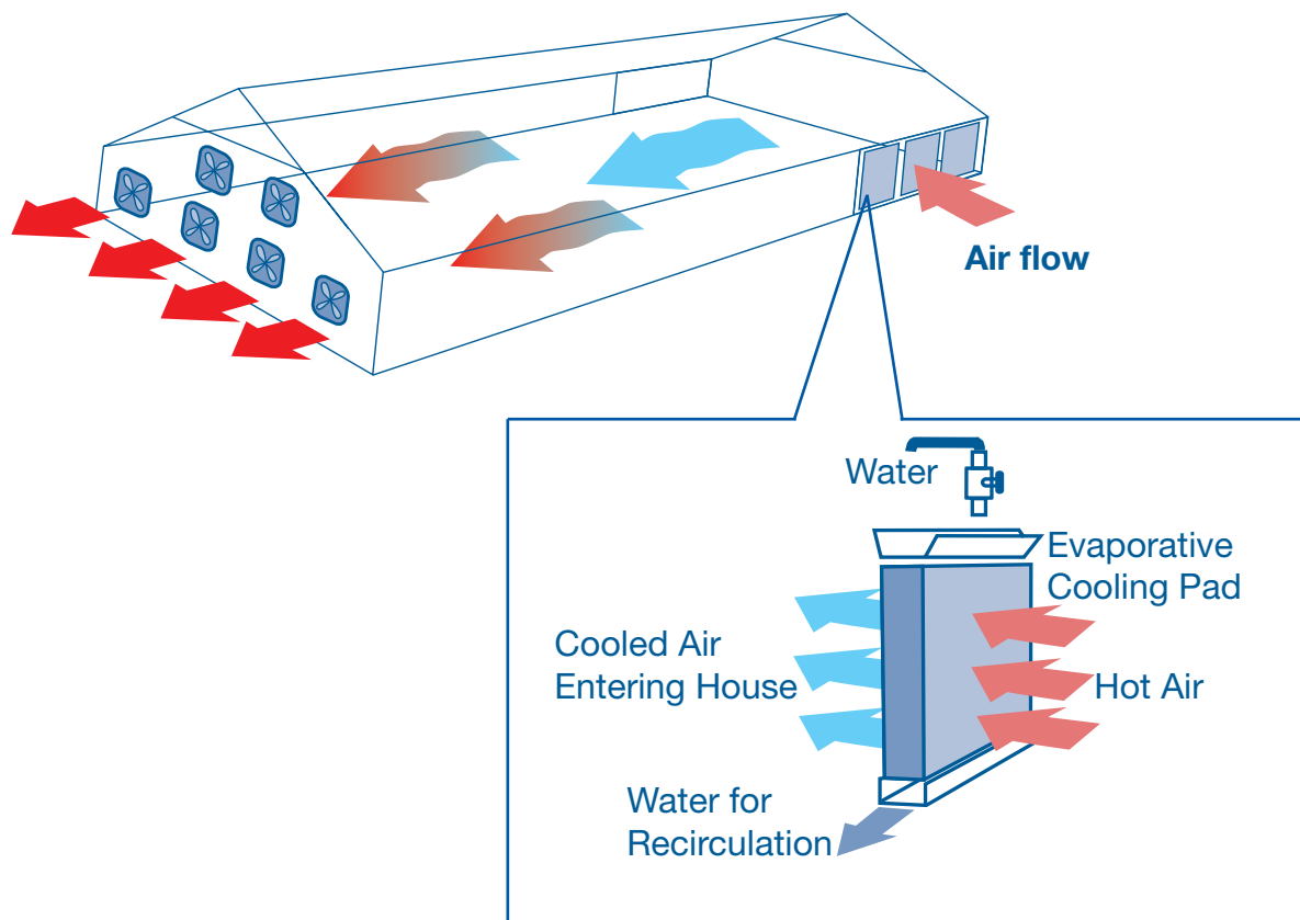
Figure 117: Pad cooling with tunnel ventilation.
