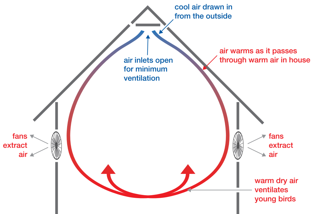
Figure 110: Diagram of reverse flow (roof inlet) ventilation.
