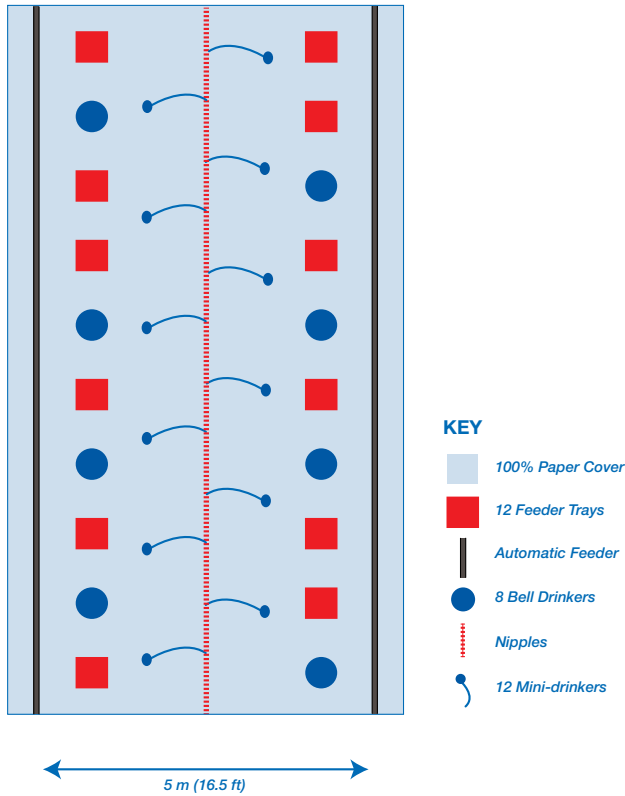
Figure 13: Typical whole-house brooding layout for 1,000 chicks.
