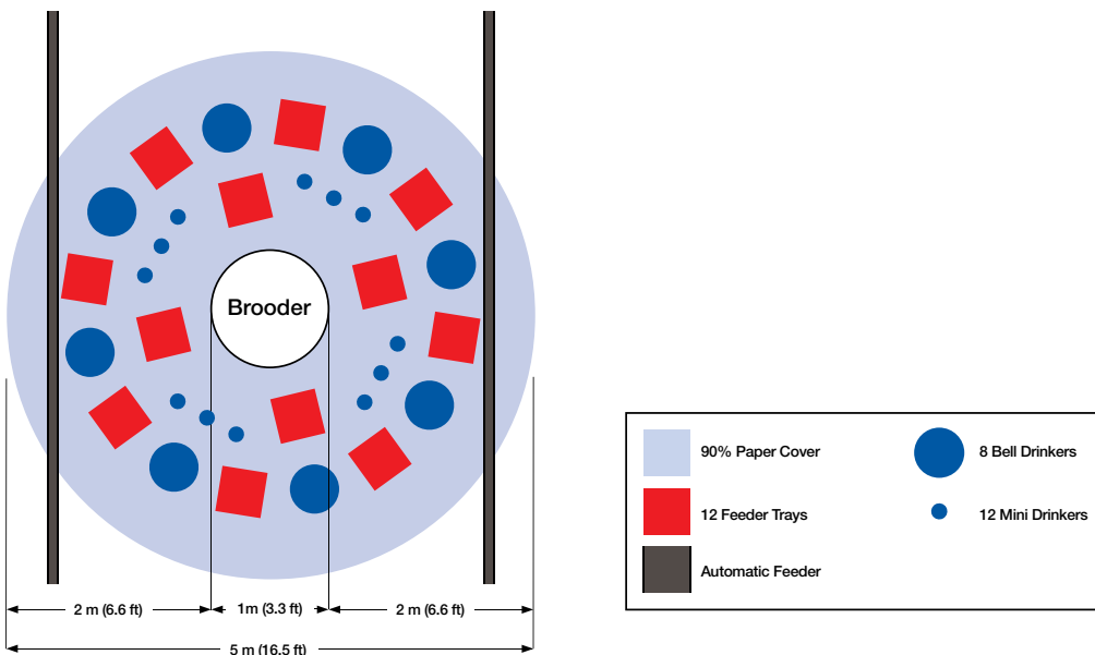
Figure 11: Example of a typical spot brooding layout (1,000 chicks).
