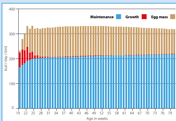
Chart 3: Daily requirements of energy of the bird
